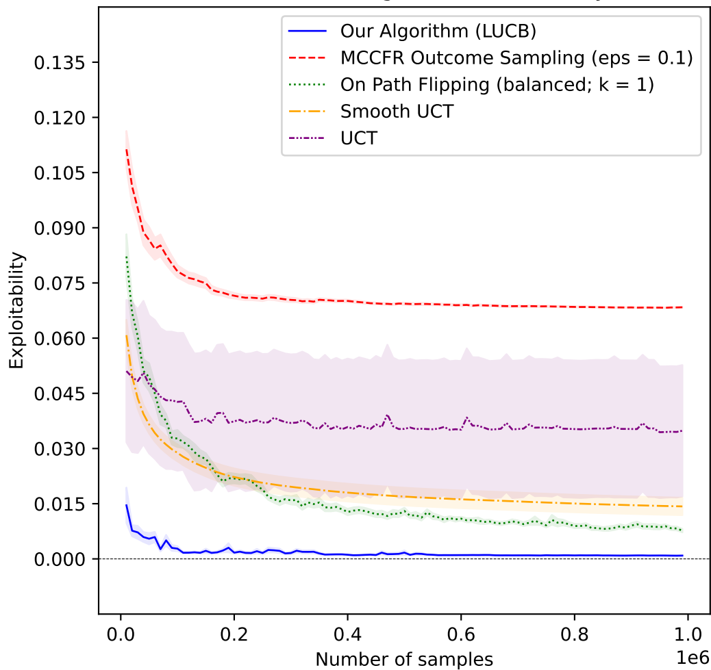
Leduc Poker, Best Algorithms (new), Player o
